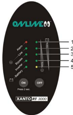
Figure 2: Control panel
