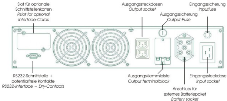
Figure 5: XANTO RT 3000 back panel
