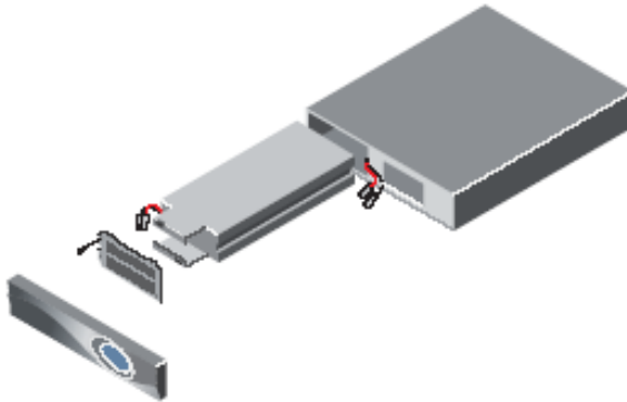
Figure 13: Hot-swap-battery for the XANTO RT 1000
