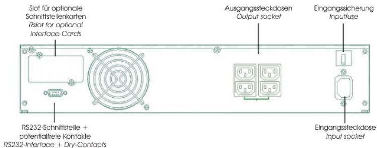
Figure 3: XANTO RT 1000 back panel
