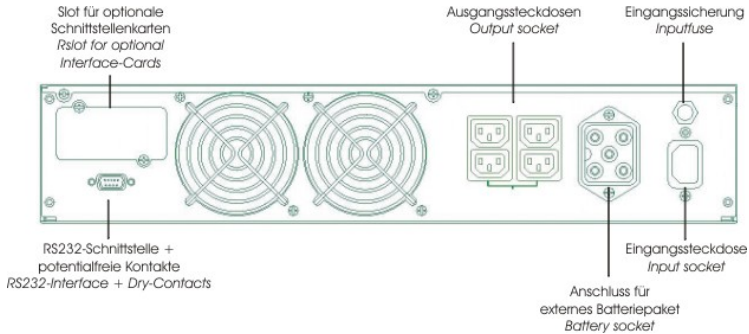
Figure 4: XANTO RT 2000 back panel
