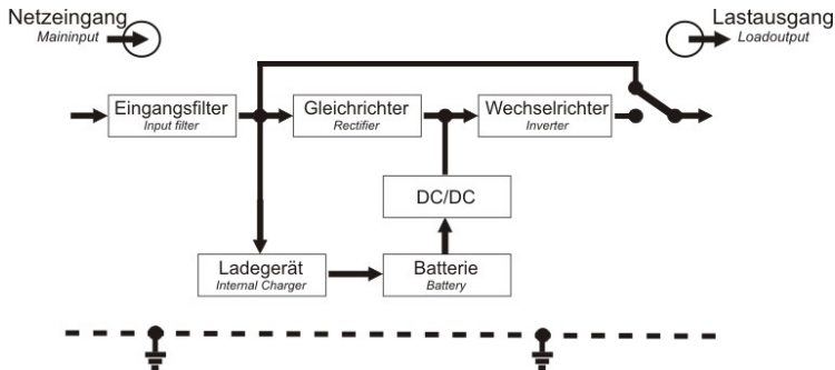
Figure 8: Block diagram
